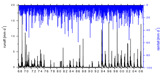
Fig. 1 Rainfall and discharge variation of the Schäfertal from 1968 until 2006
