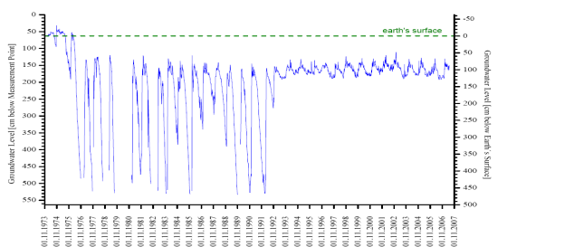
Fig. 2 Modification of groundwater level and discharge and runoff generation by mining activities
